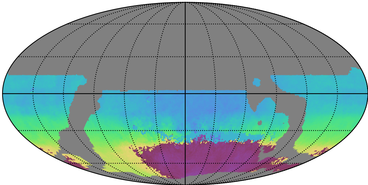
weather_cloudso10v3.4_10yrs WFD r band: AngleMean rotSkyPos
