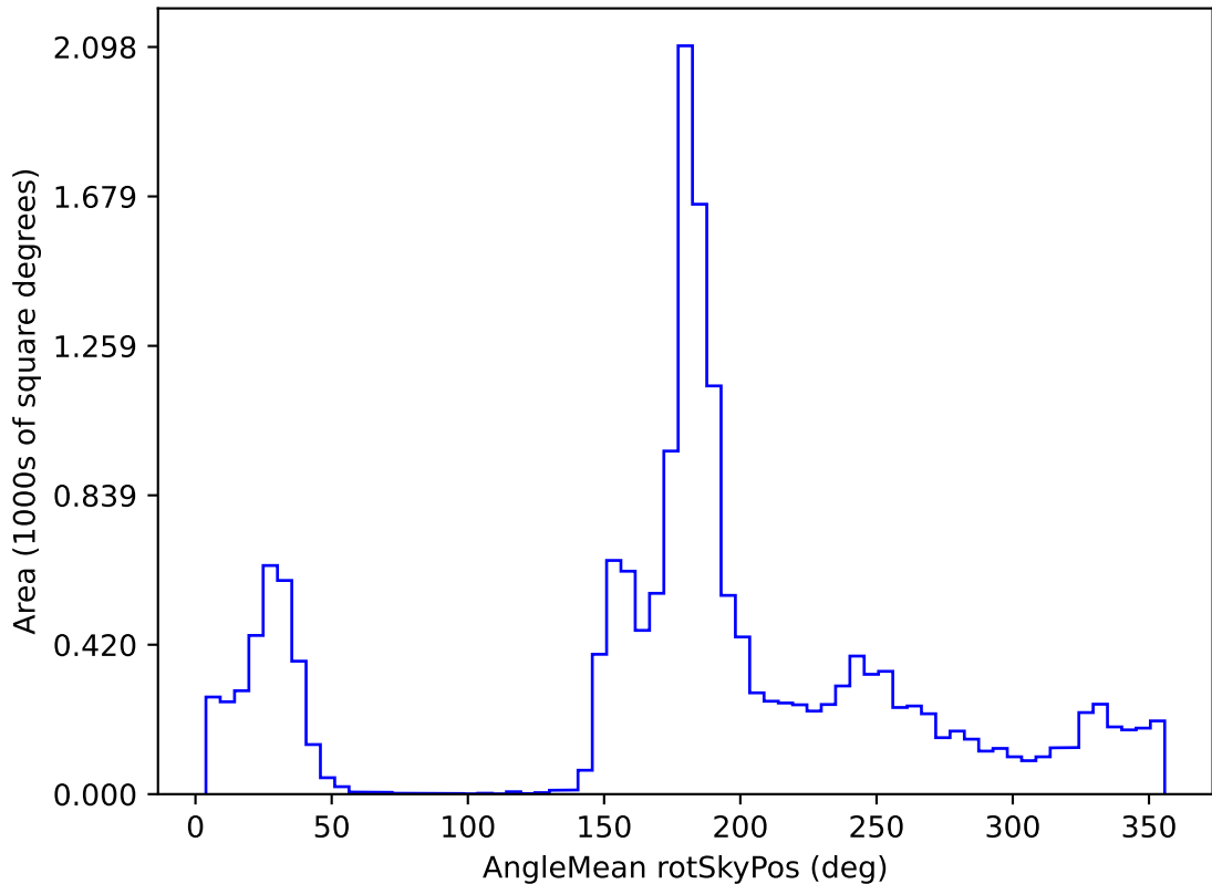
weather_cloudso10v3.4_10yrs WFD r band: AngleMean rotSkyPos
