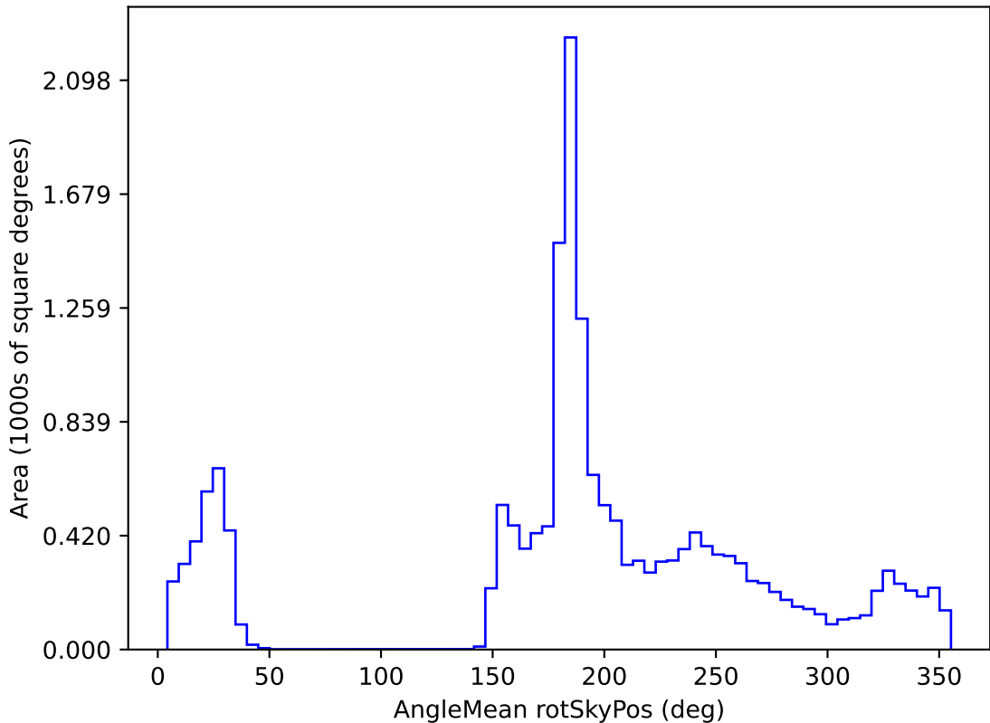
weather_cloudso10v3.4_10yrs WFD all bands: AngleMean rotSkyPos
