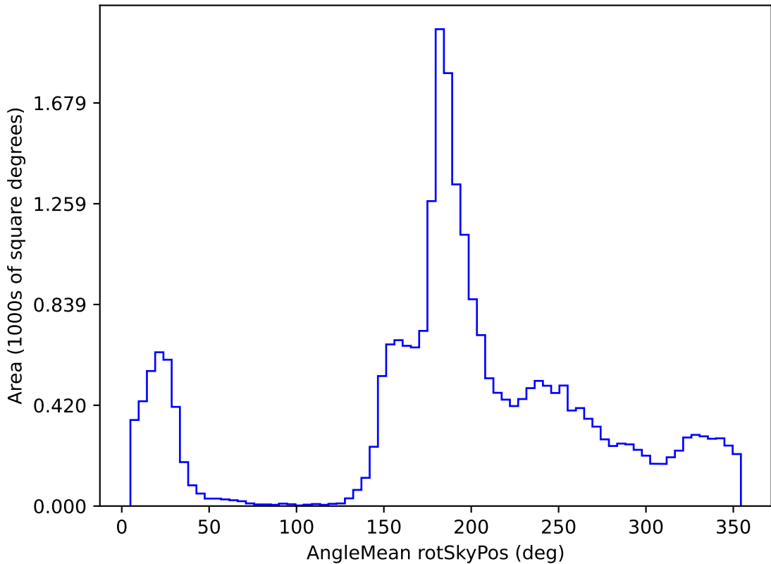
weather_cloudso10v3.4_10yrs All sky z band: AngleMean rotSkyPos
