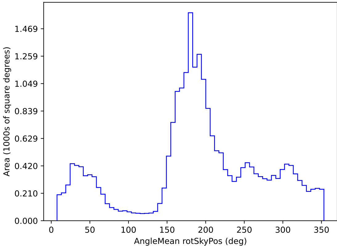
weather_cloudso10v3.4_10yrs All sky u band: AngleMean rotSkyPos
