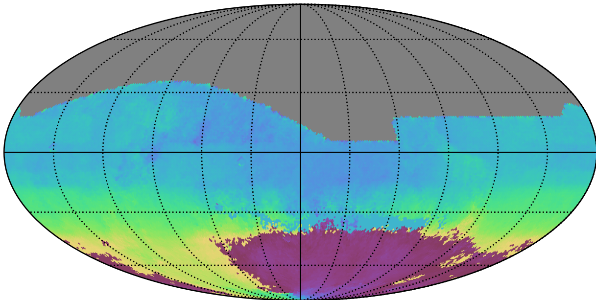
weather_cloudso10v3.4_10yrs All sky r band: AngleMean rotSkyPos
