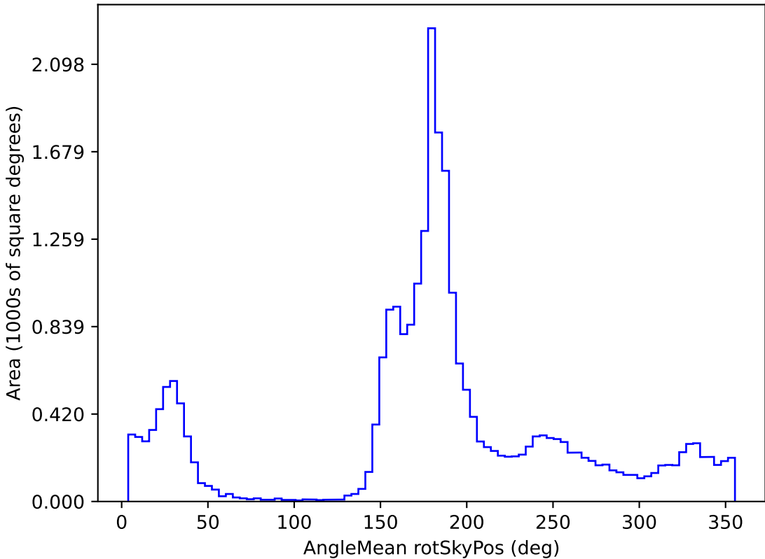
weather_cloudso10v3.4_10yrs All sky r band: AngleMean rotSkyPos
