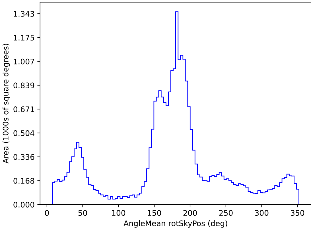
weather_cloudso10v3.4_10yrs All sky g band: AngleMean rotSkyPos
