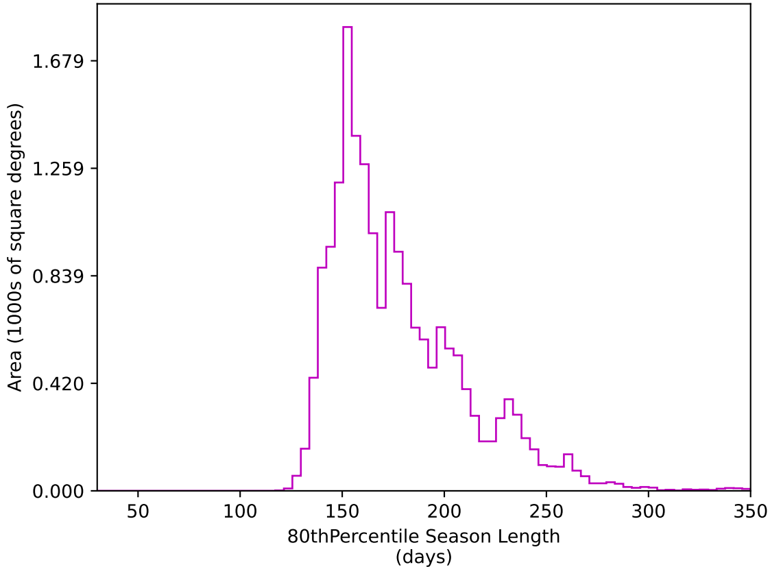
weather_cloudso10v3.4_10yrs WFD z band: 80thPercentile Season Length
