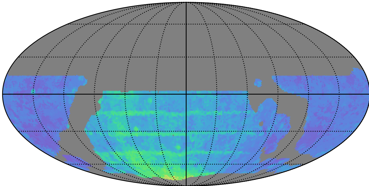
weather_cloudso10v3.4_10yrs WFD y band: 80thPercentile Season Length
