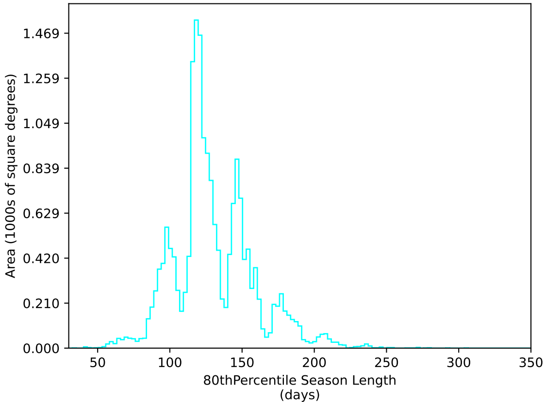
weather_cloudso10v3.4_10yrs WFD u band: 80thPercentile Season Length
