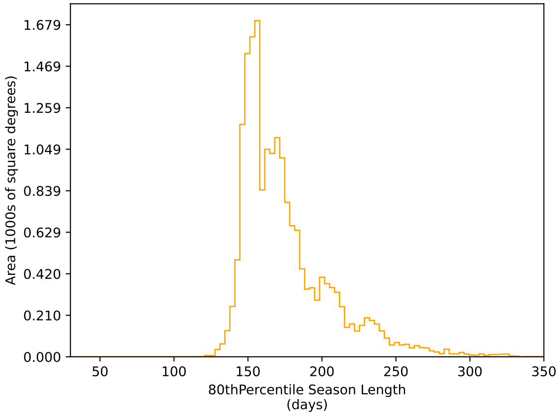
weather_cloudso10v3.4_10yrs WFD r band: 80thPercentile Season Length
