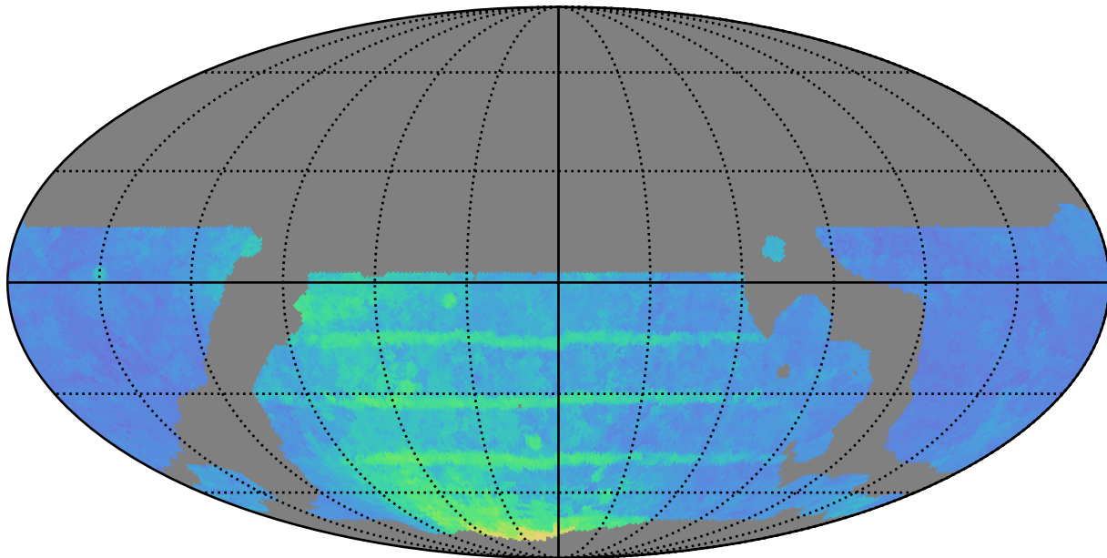
weather_cloudso10v3.4_10yrs WFD i band: 80thPercentile Season Length
