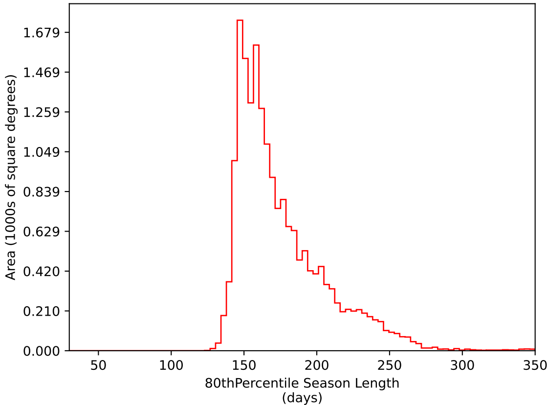
weather_cloudso10v3.4_10yrs WFD i band: 80thPercentile Season Length
