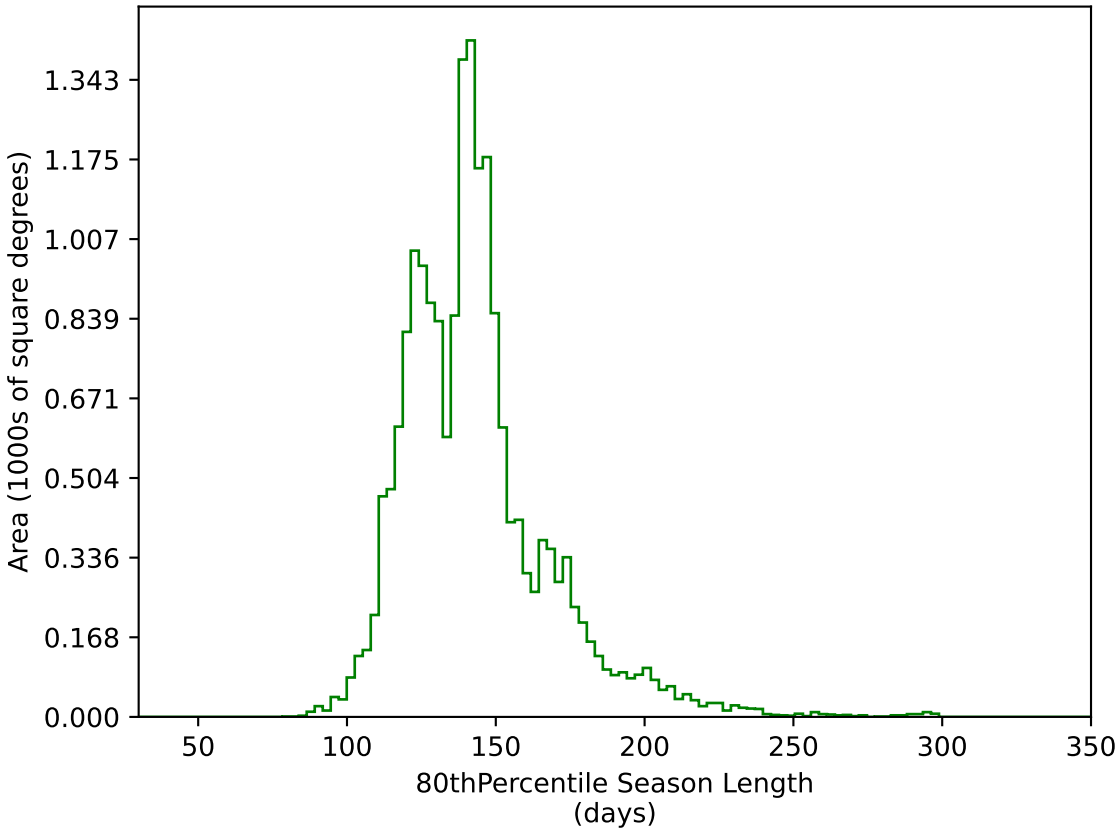
weather_cloudso10v3.4_10yrs WFD g band: 80thPercentile Season Length
