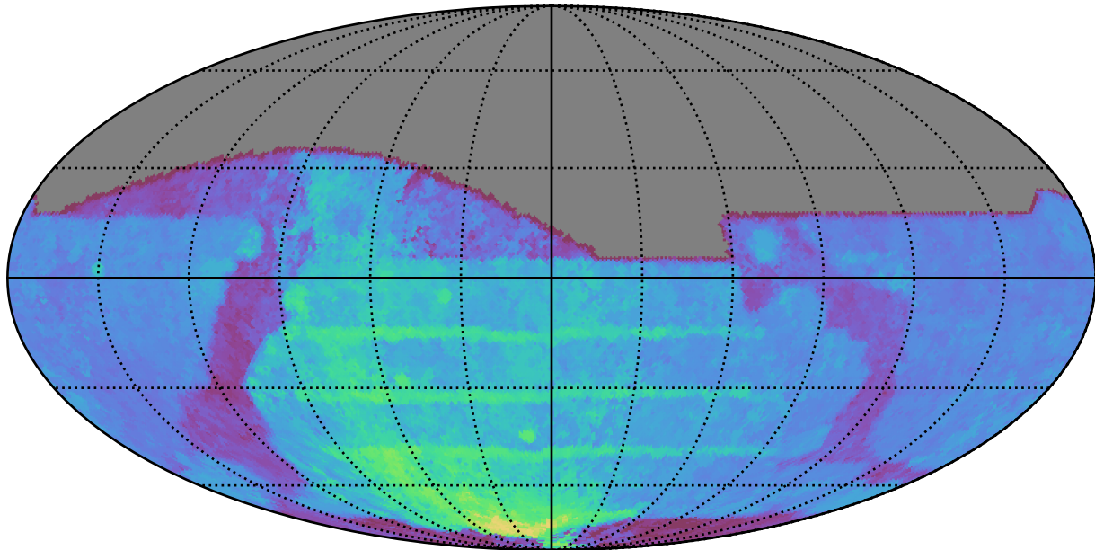
weather_cloudso10v3.4_10yrs All sky z band: 80thPercentile Season Length
