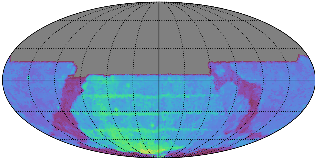
weather_cloudso10v3.4_10yrs All sky y band: 80thPercentile Season Length
