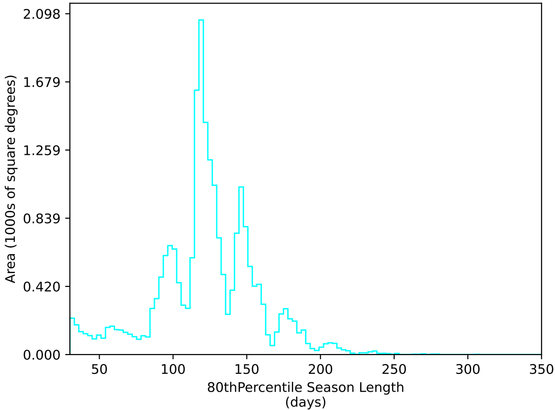
weather_cloudso10v3.4_10yrs All sky u band: 80thPercentile Season Length
