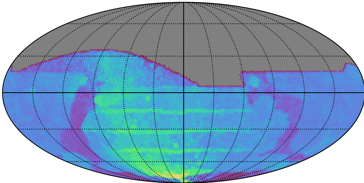
weather_cloudso10v3.4_10yrs All sky i band: 80thPercentile Season Length
