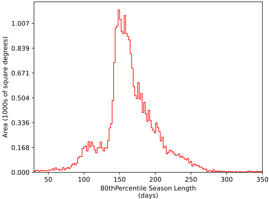
weather_cloudso10v3.4_10yrs All sky i band: 80thPercentile Season Length
