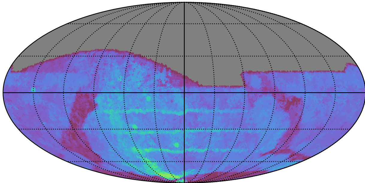
weather_cloudso10v3.4_10yrs All sky g band: 80thPercentile Season Length
