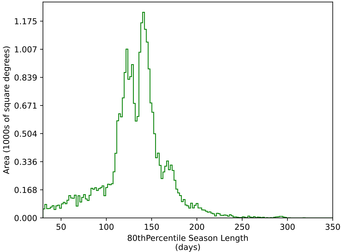
weather_cloudso10v3.4_10yrs All sky g band: 80thPercentile Season Length
