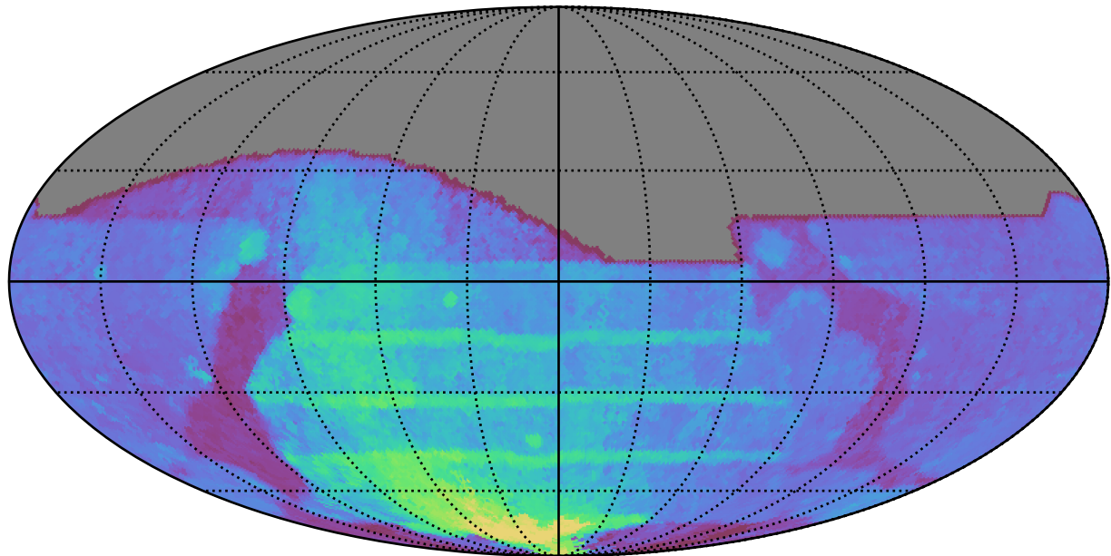
weather_cloudso10v3.4_10yrs All sky all bands: 80thPercentile Season Length
