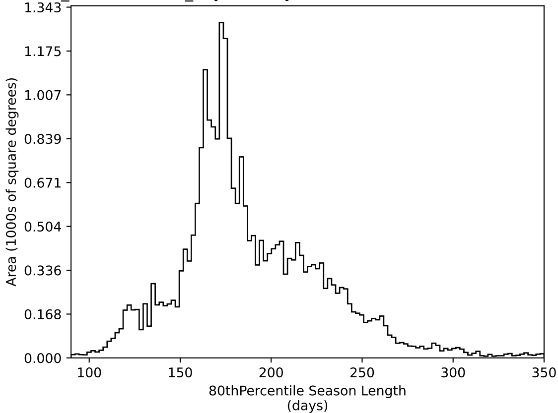
weather_cloudso10v3.4_10yrs All sky all bands: 80thPercentile Season Length
