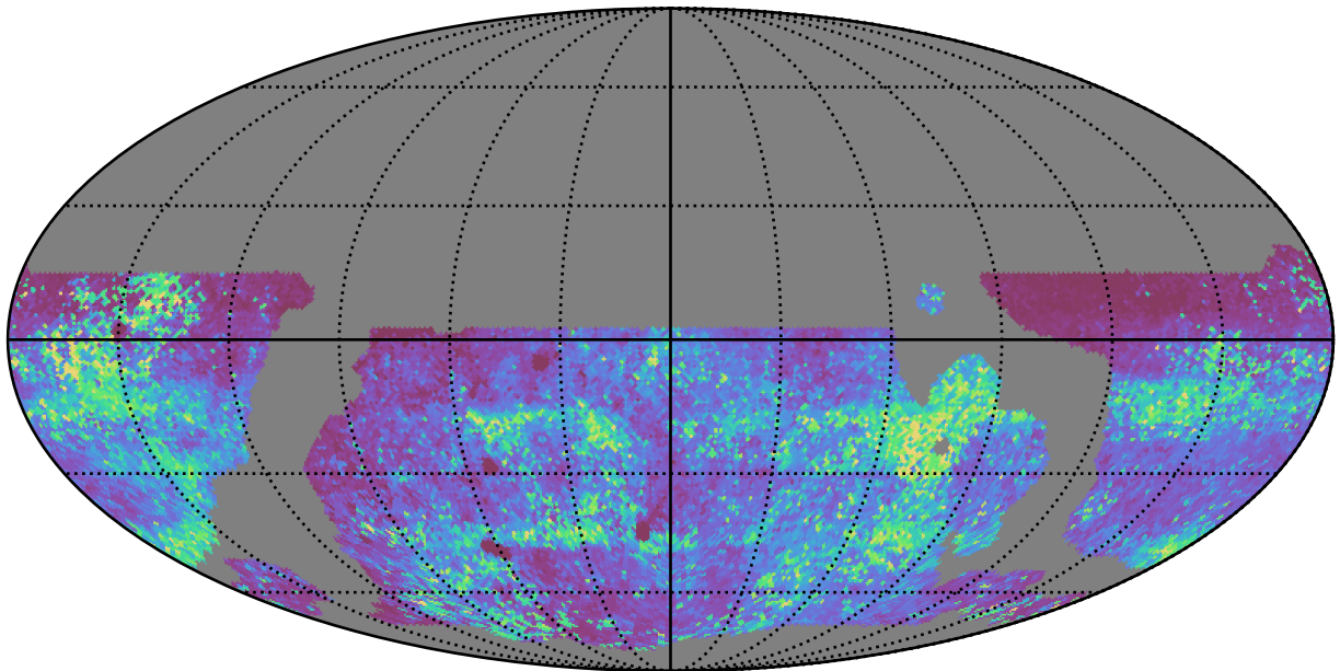
weather_cloudso10v3.4_10yrs WFD zy bands: 75th Percentile Intranight Timespan
