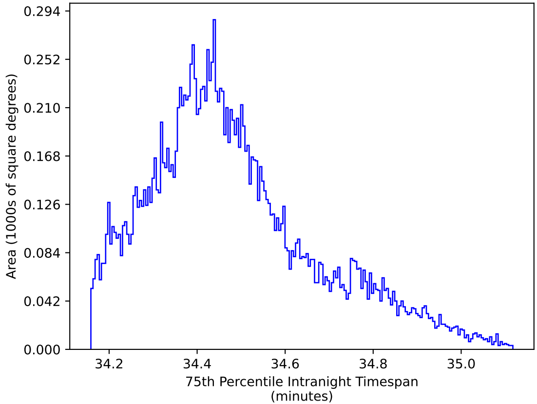
weather_cloudso10v3.4_10yrs WFD zy bands: 75th Percentile Intranight Timespan
