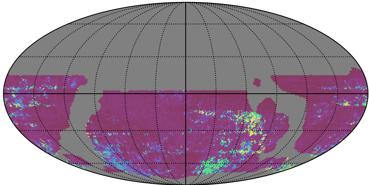
weather_cloudso10v3.4_10yrs WFD z band: 75th Percentile Intranight Timespan
