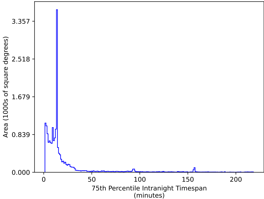
weather_cloudso10v3.4_10yrs WFD z band: 75th Percentile Intranight Timespan
