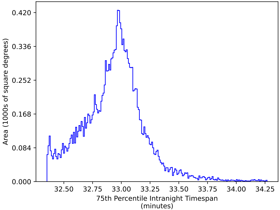
weather_cloudso10v3.4_10yrs WFD y band: 75th Percentile Intranight Timespan
