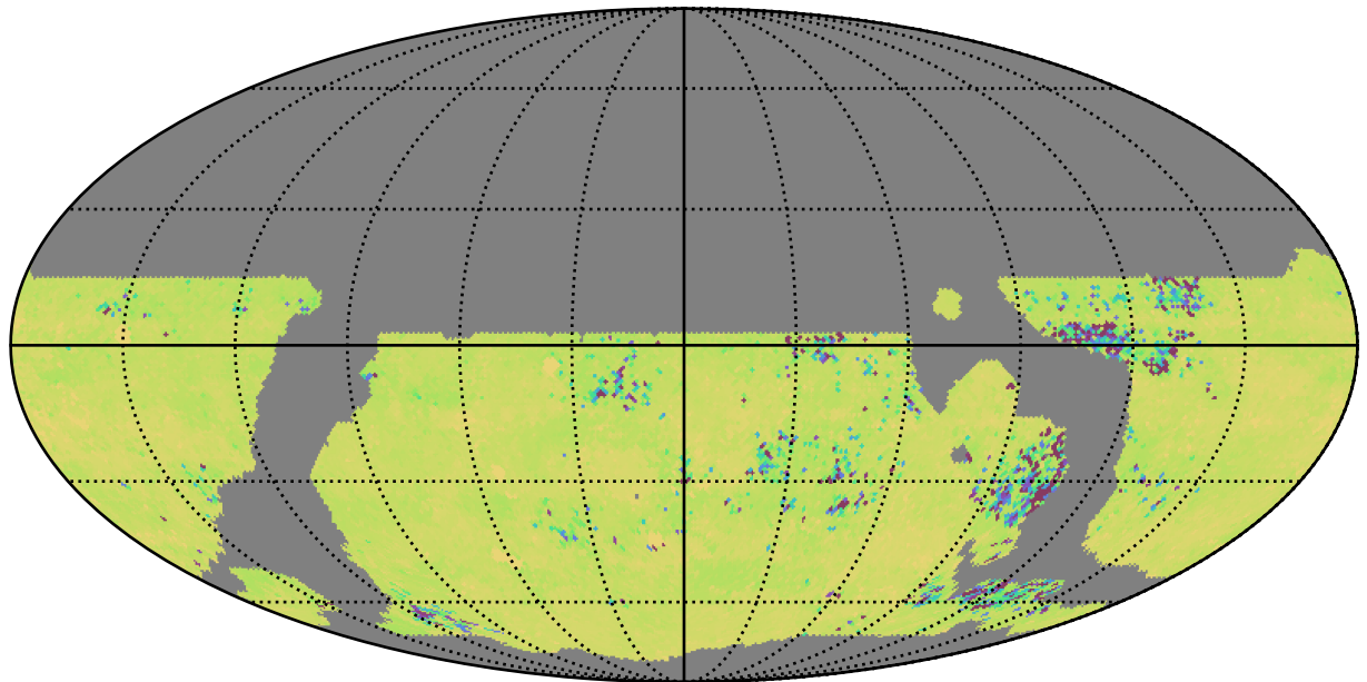
weather_cloudso10v3.4_10yrs WFD ug bands: 75th Percentile Intranight Timespan
