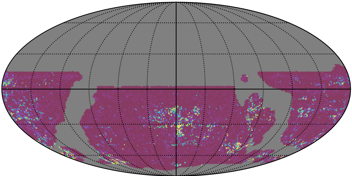
weather_cloudso10v3.4_10yrs WFD u band: 75th Percentile Intranight Timespan
