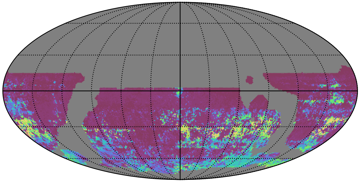
weather_cloudso10v3.4_10yrs WFD r band: 75th Percentile Intranight Timespan
