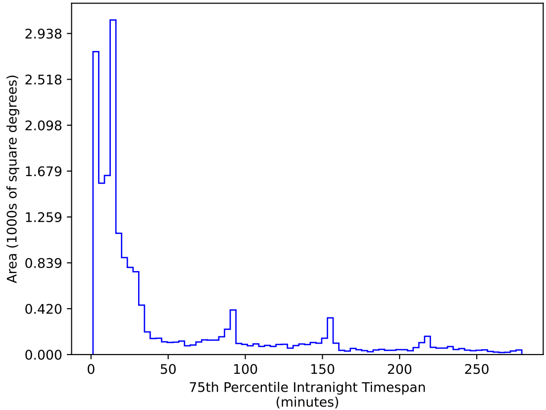
weather_cloudso10v3.4_10yrs WFD r band: 75th Percentile Intranight Timespan
