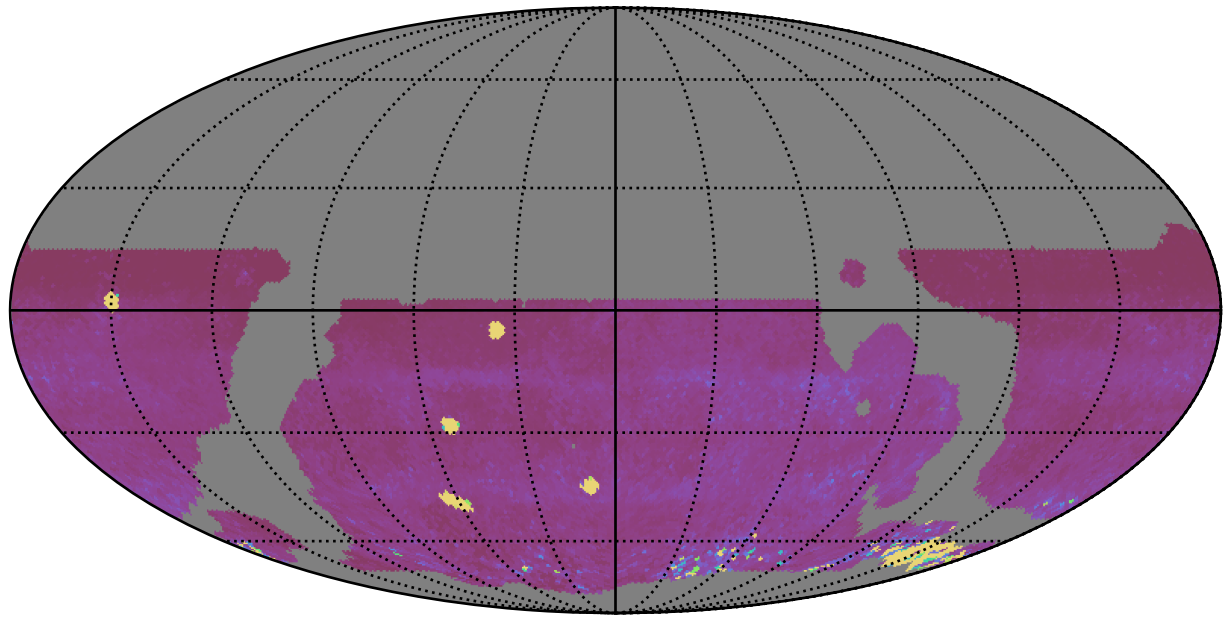
weather_cloudso10v3.4_10yrs WFD iz bands: 75th Percentile Intranight Timespan
