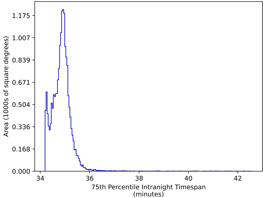
weather_cloudso10v3.4_10yrs WFD iz bands: 75th Percentile Intranight Timespan
