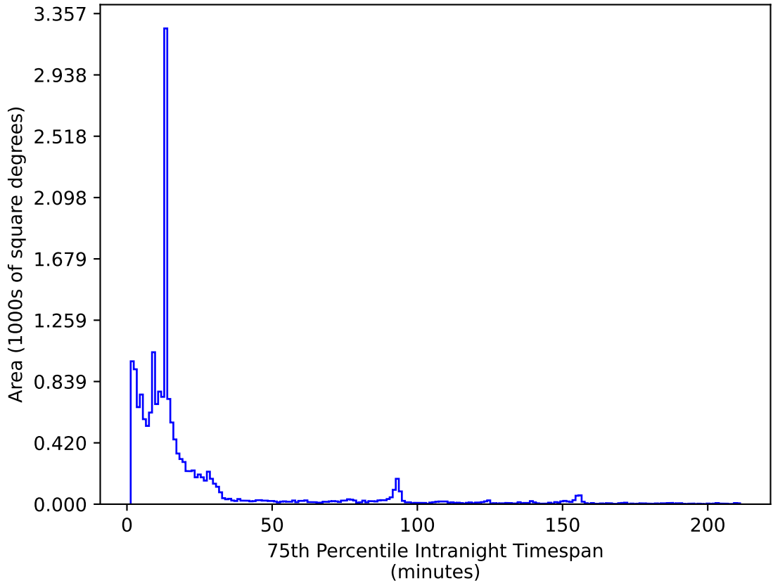
weather_cloudso10v3.4_10yrs WFD i band: 75th Percentile Intranight Timespan
