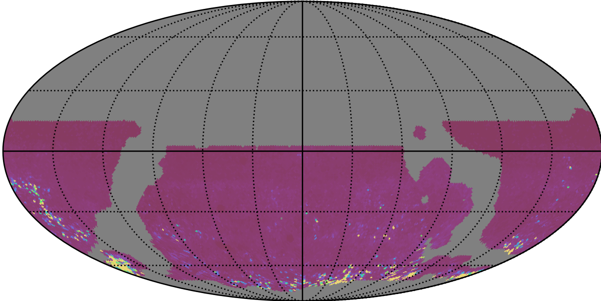
weather_cloudso10v3.4_10yrs WFD gr bands: 75th Percentile Intranight Timespan
