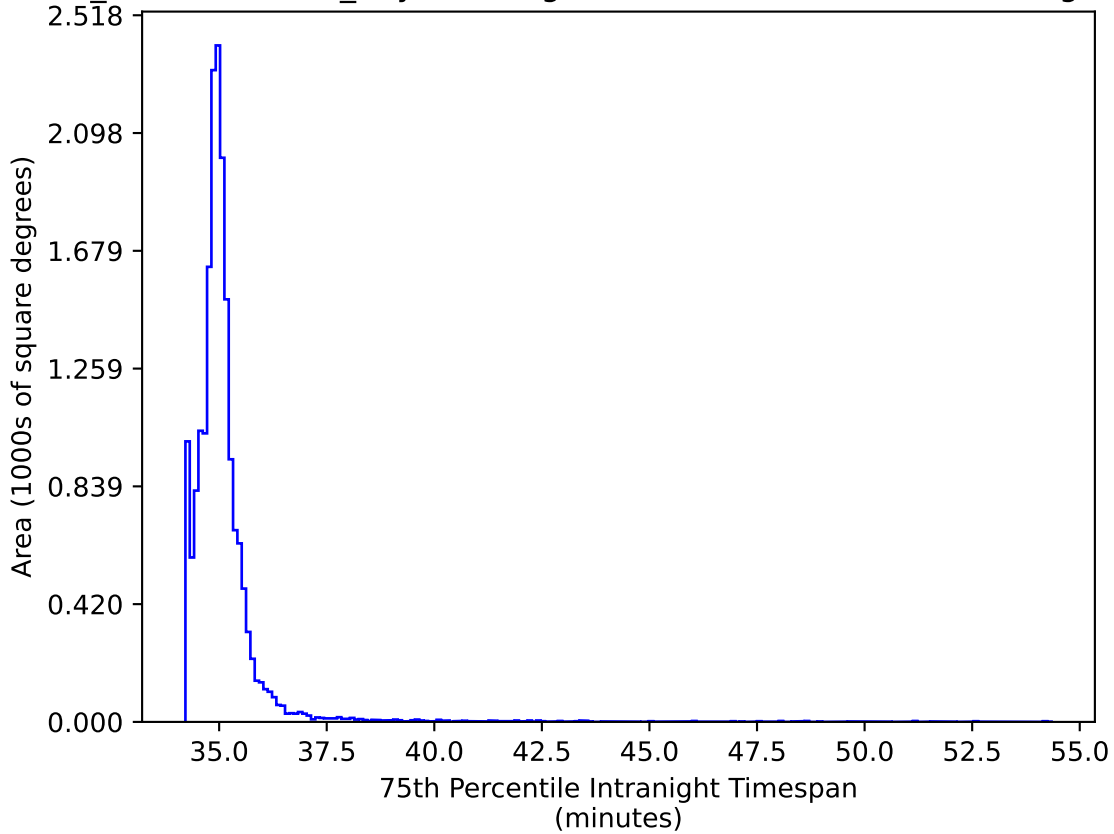
weather_cloudso10v3.4_10yrs WFD gr bands: 75th Percentile Intranight Timespan
