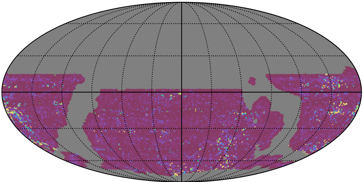
weather_cloudso10v3.4_10yrs WFD g band: 75th Percentile Intranight Timespan
