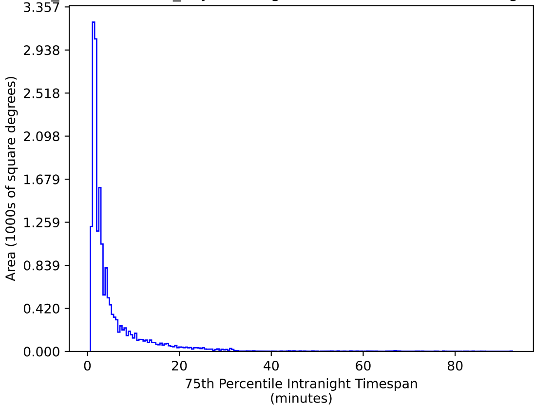
weather_cloudso10v3.4_10yrs WFD g band: 75th Percentile Intranight Timespan
