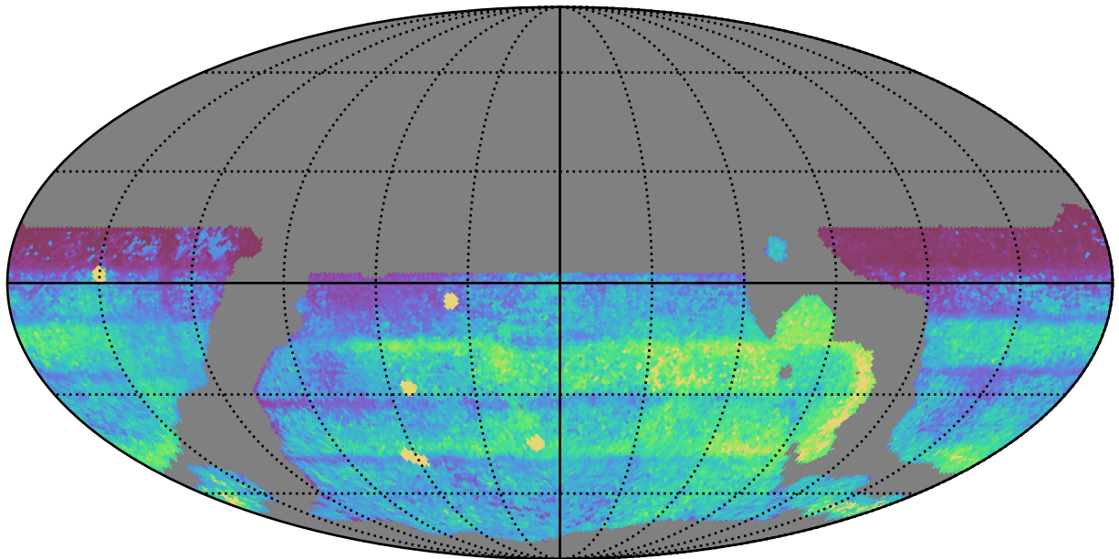
weather_cloudso10v3.4_10yrs WFD all bands: 75th Percentile Intranight Timespan
