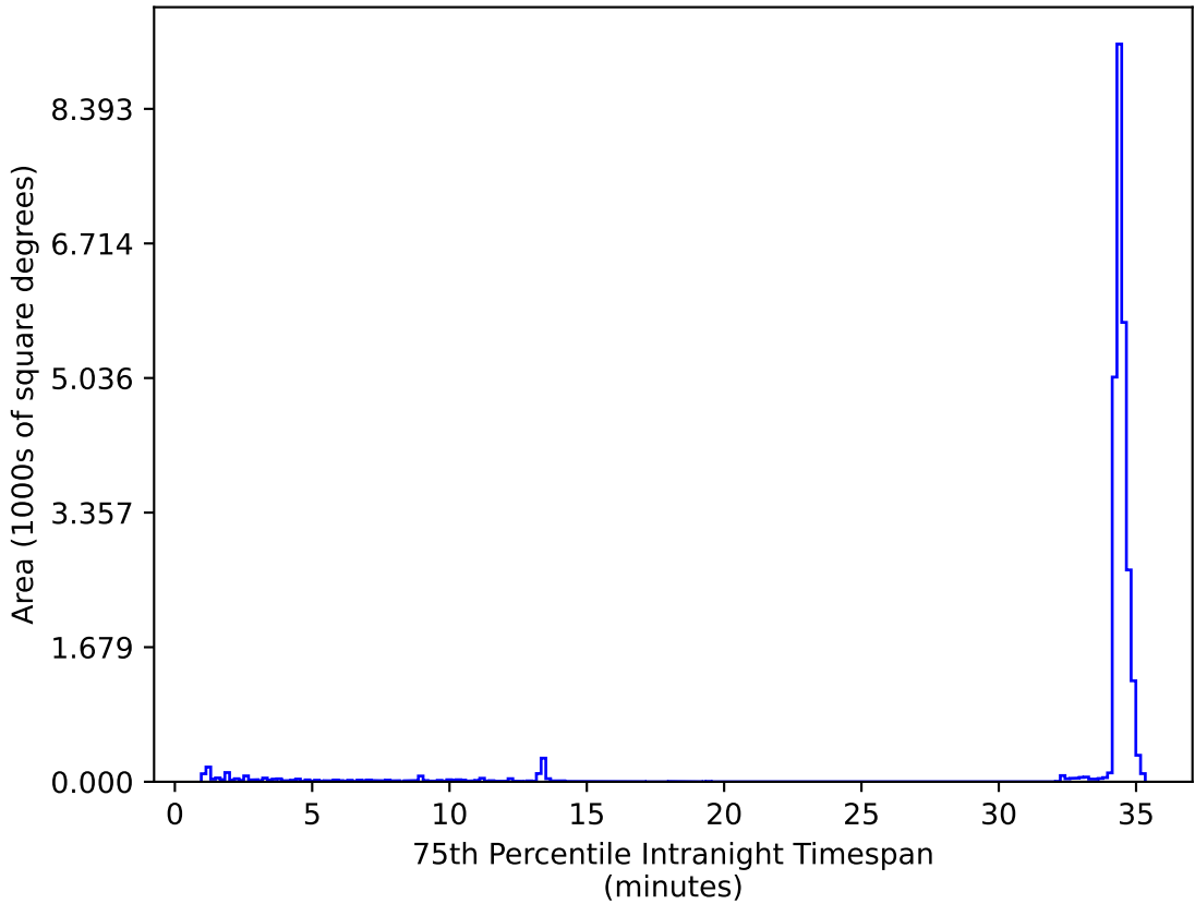
weather_cloudso10v3.4_10yrs All sky zy bands: 75th Percentile Intranight Timespan
