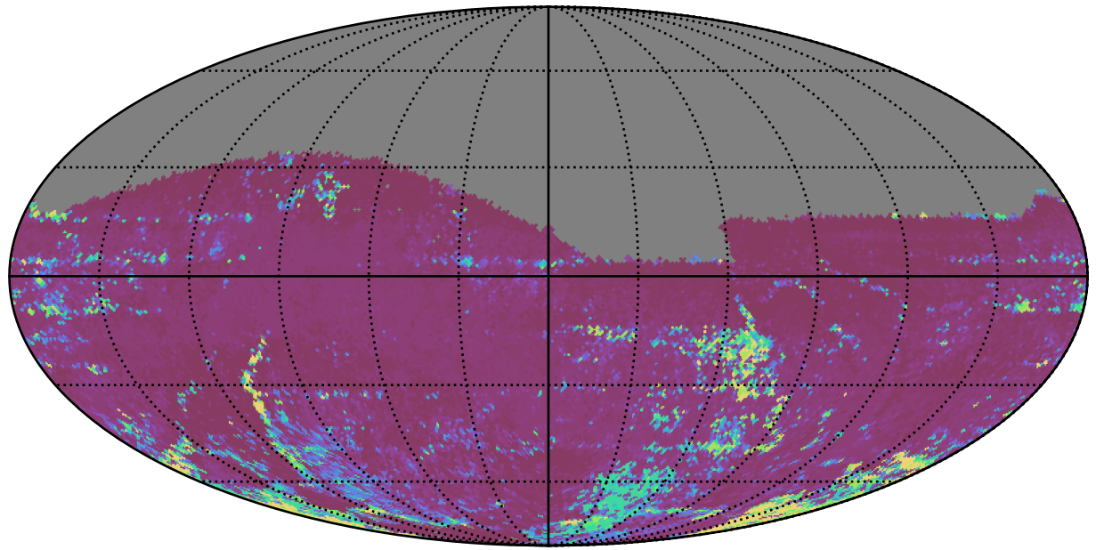
weather_cloudso10v3.4_10yrs All sky z band: 75th Percentile Intranight Timespan
