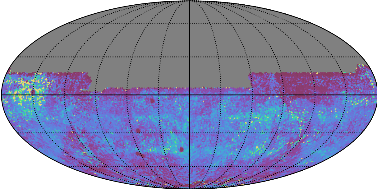
weather_cloudso10v3.4_10yrs All sky y band: 75th Percentile Intranight Timespan
