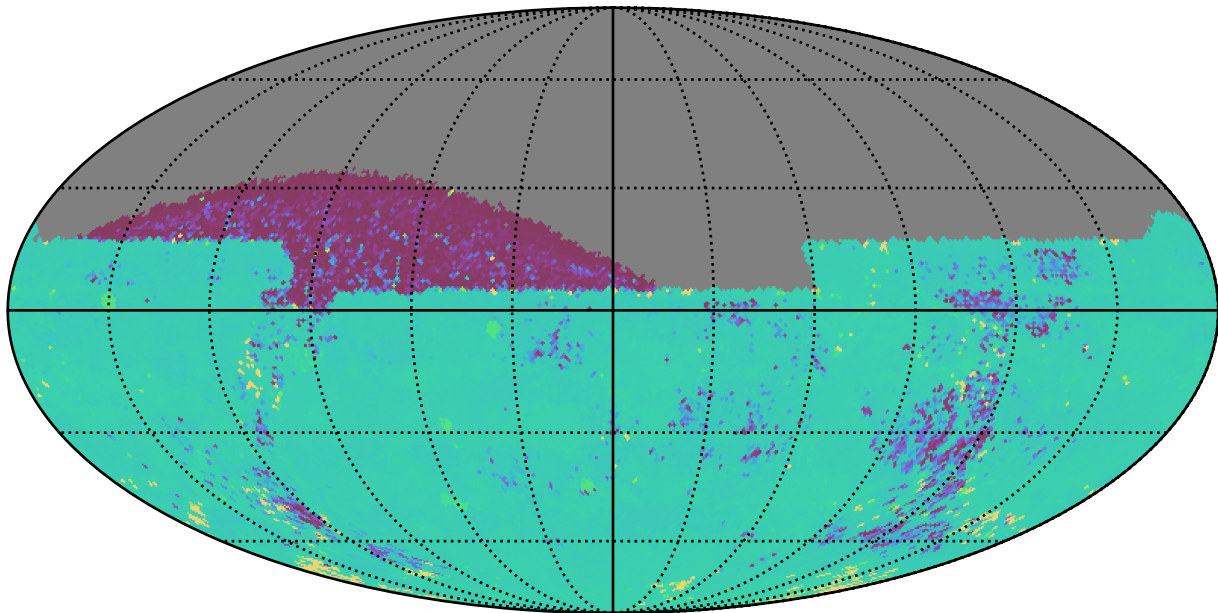
weather_cloudso10v3.4_10yrs All sky ug bands: 75th Percentile Intranight Timespan
