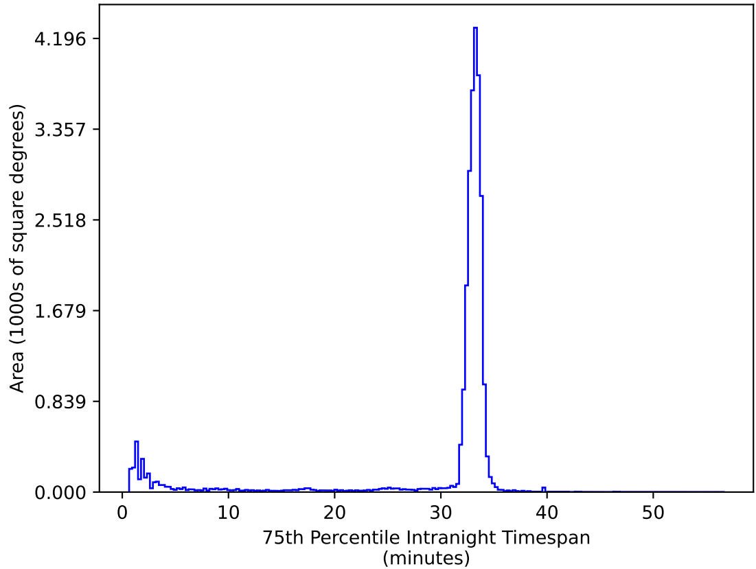
weather_cloudso10v3.4_10yrs All sky ug bands: 75th Percentile Intranight Timespan
