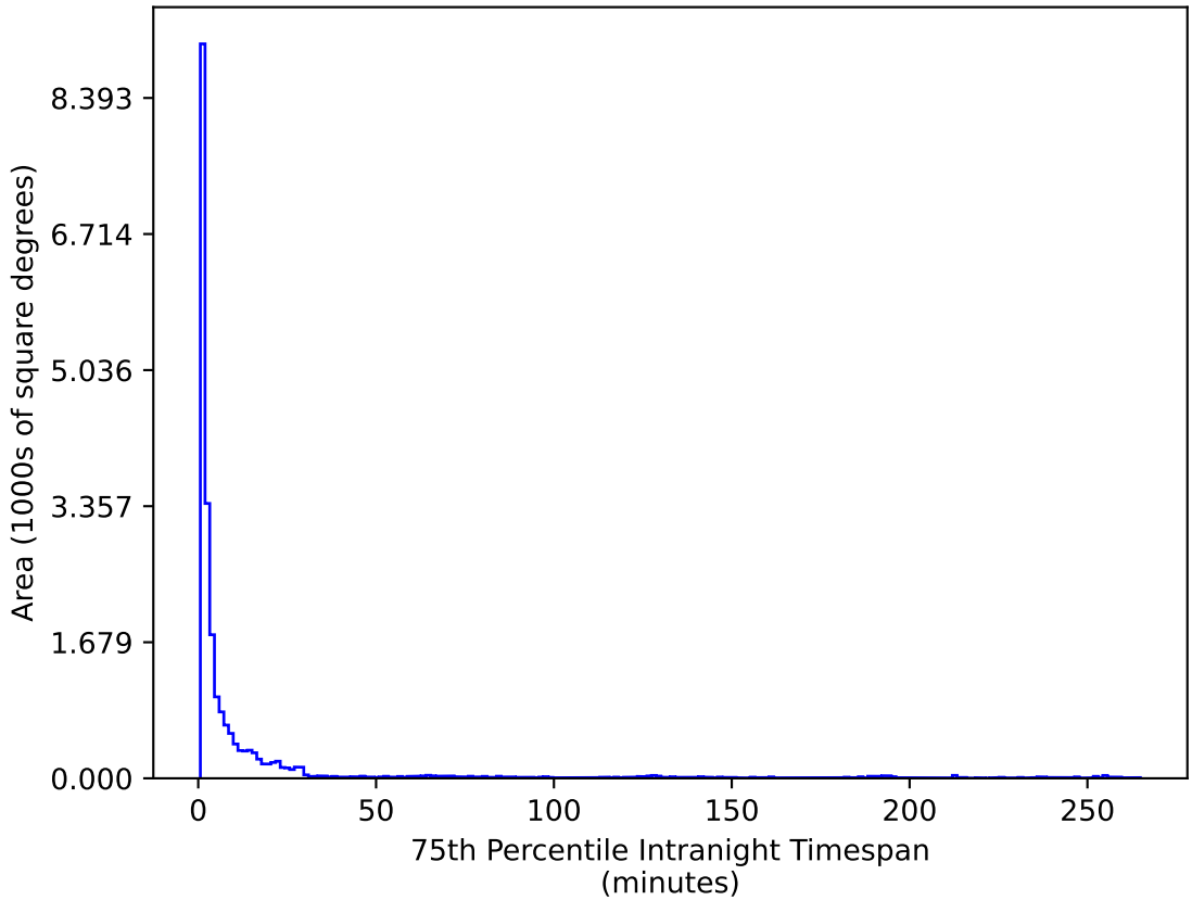
weather_cloudso10v3.4_10yrs All sky u band: 75th Percentile Intranight Timespan
