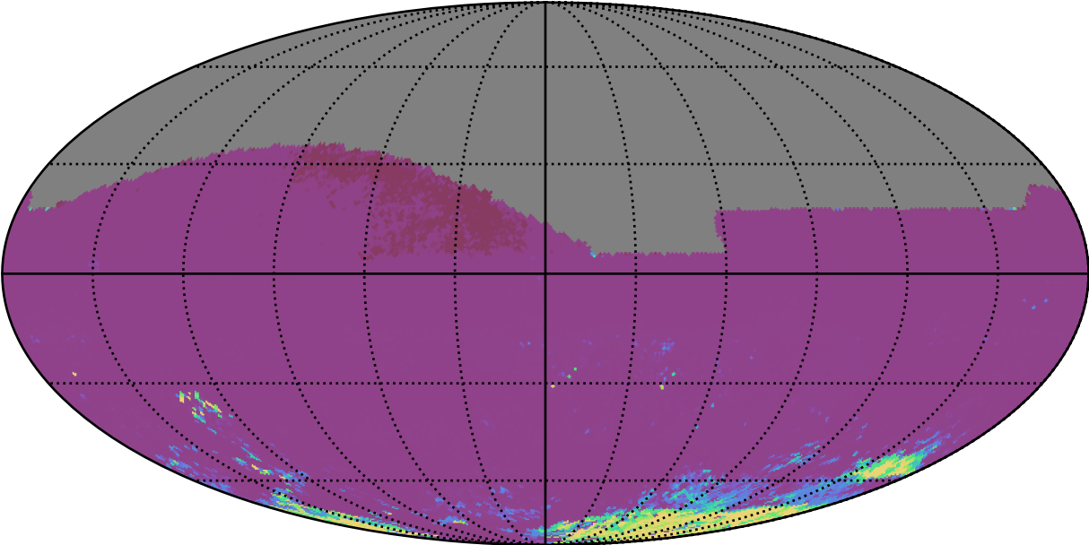
weather_cloudso10v3.4_10yrs All sky ri bands: 75th Percentile Intranight Timespan
