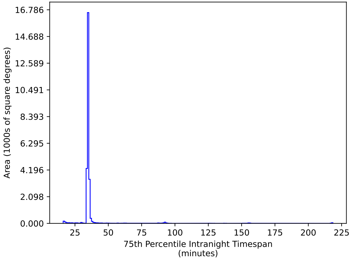
weather_cloudso10v3.4_10yrs All sky ri bands: 75th Percentile Intranight Timespan
