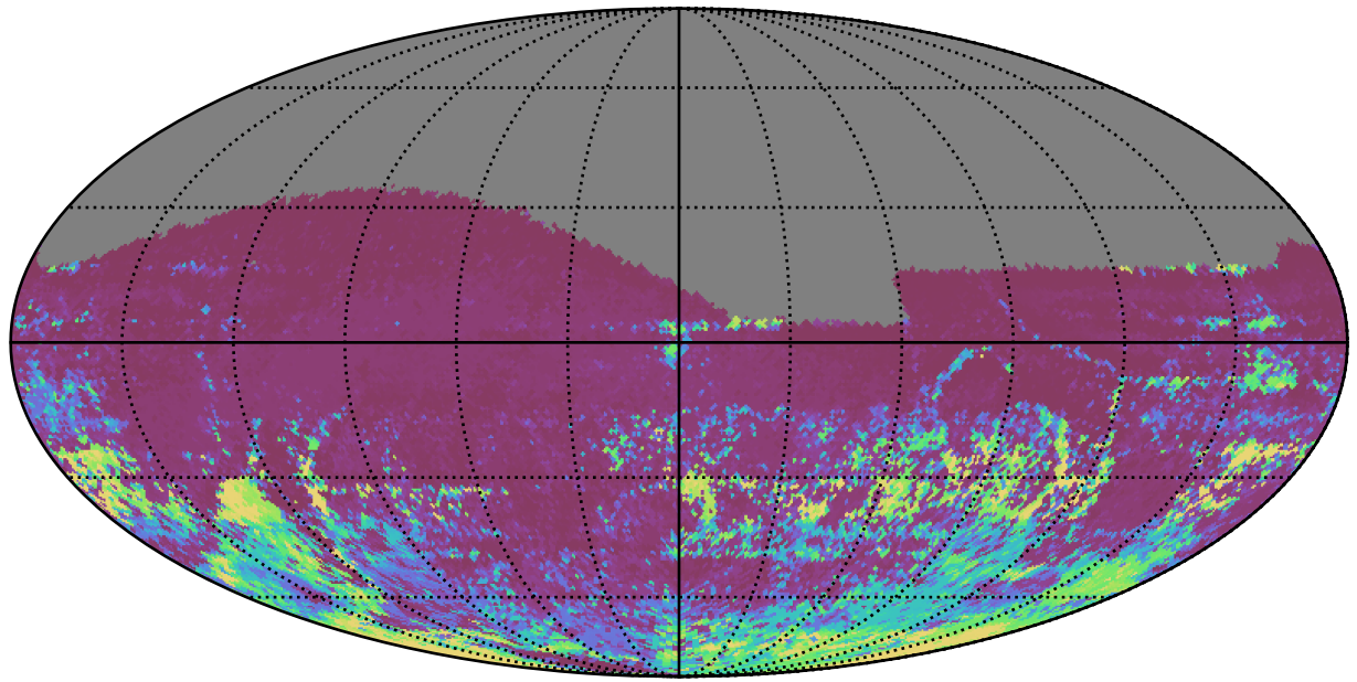
weather_cloudso10v3.4_10yrs All sky r band: 75th Percentile Intranight Timespan
